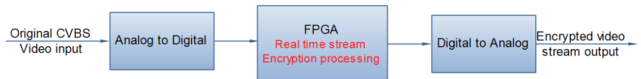
Schematic diagram of real-time encryption processing for CVBS video streams
