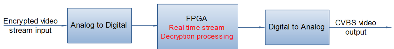
Schematic diagram of real time decryption CVBS video stream
